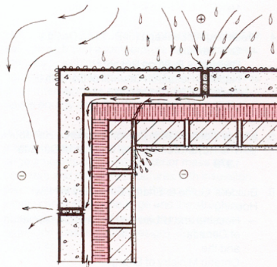
A. Corner conditions defeat rainscreen
