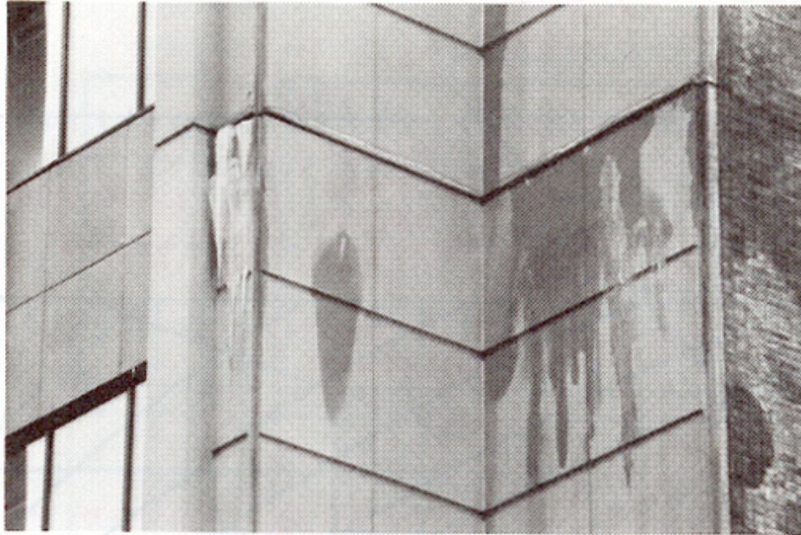
Figure 2.10 Exfiltration/Condensation
