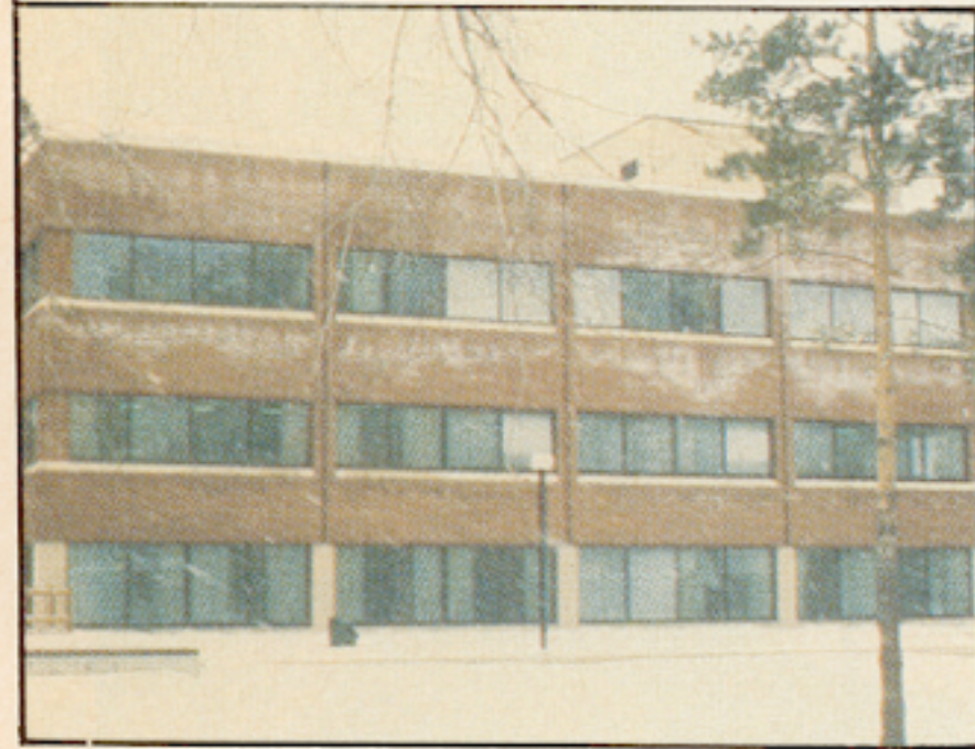
Efflorescence on masonry (Photo I)
