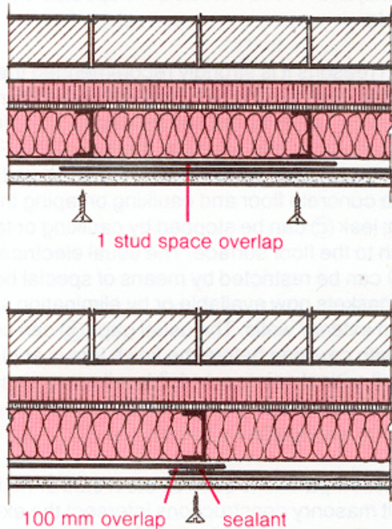
Figure 2.17 Recommended Joints in Polyethelene Air/Vapour Barrier
