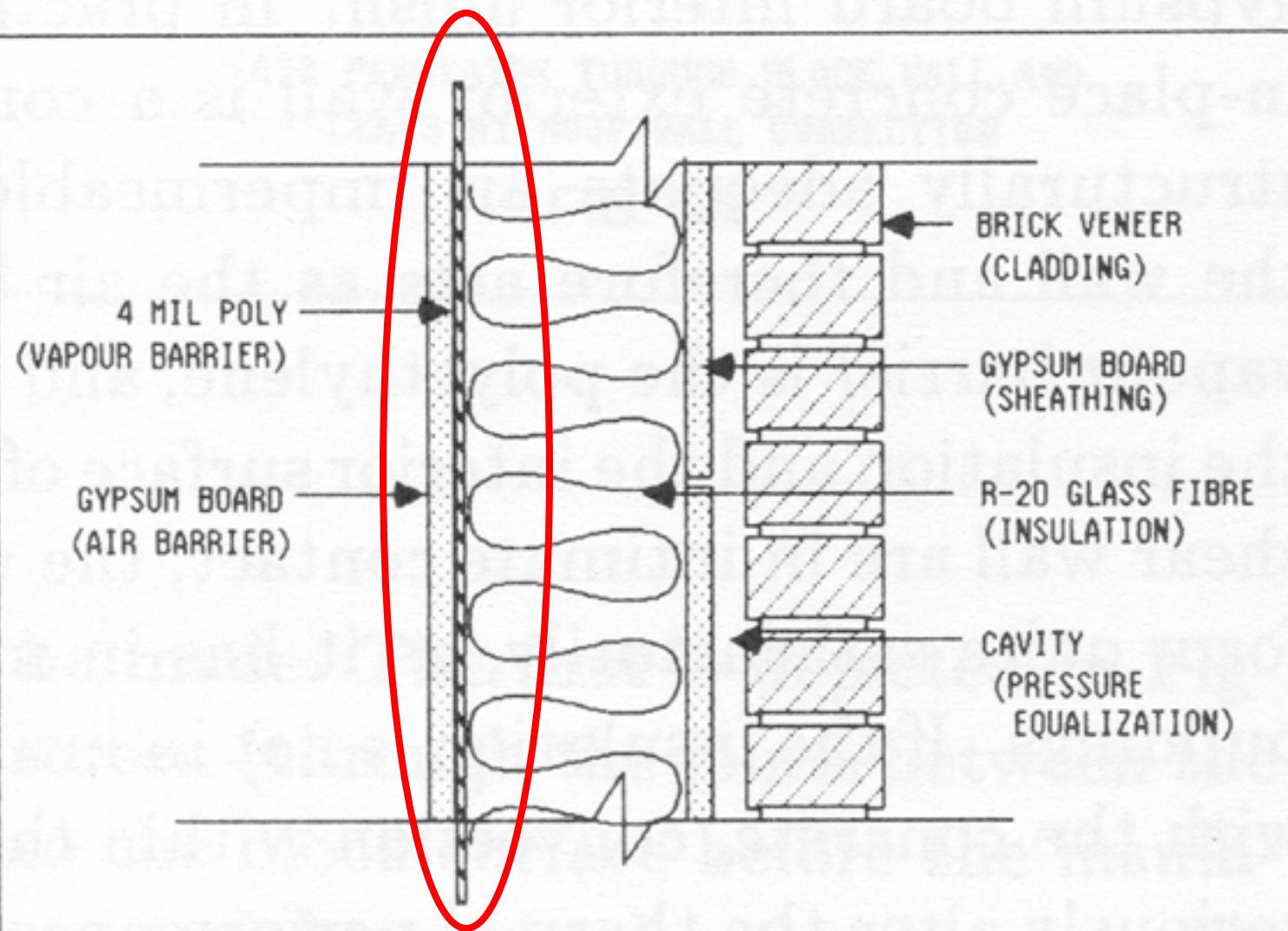
SEPARATE AIR AND VAPOUR BARRIERS
