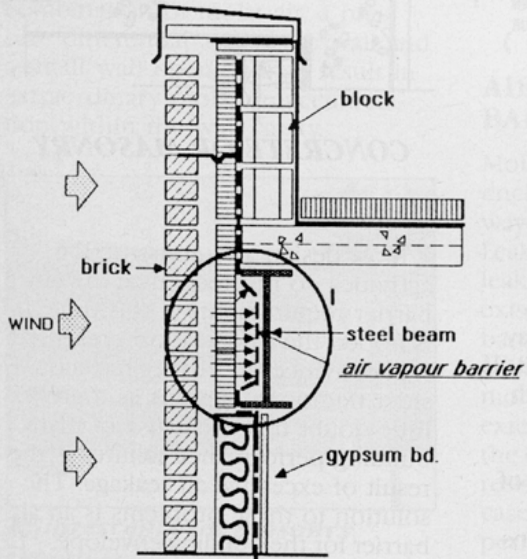
AIR BARRIER RESISTS DISPLACEMENT
