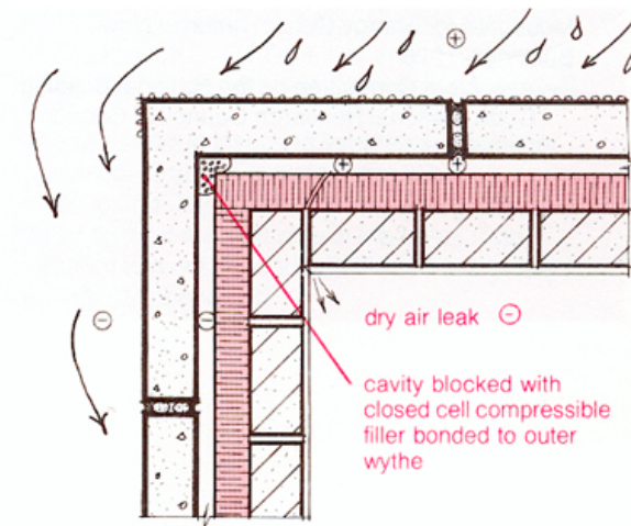
B. With corner blocking, rain screen functions properly
