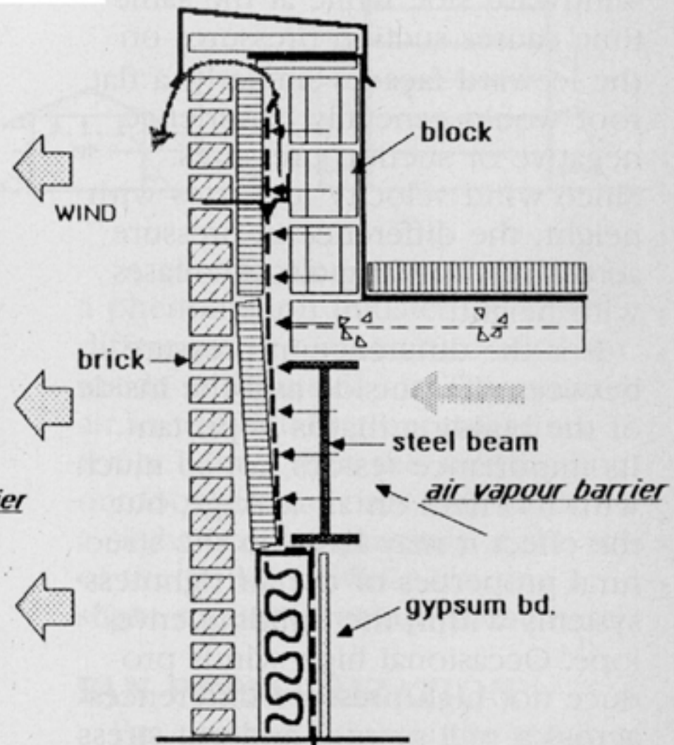
AIR BARRIER DISPLACEMENT
