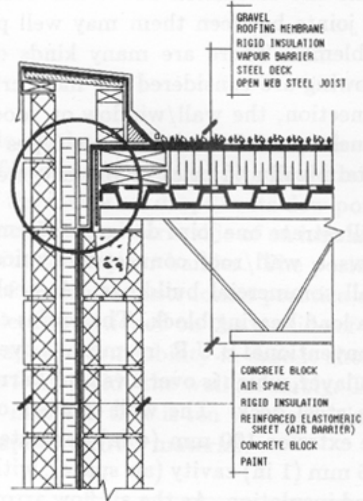
ROOF MEMBRANE (AIR BARRIER) IS CONNECTED TO ELASTOMERIC SHEET (AIR BARRIER) FIG. 9C
