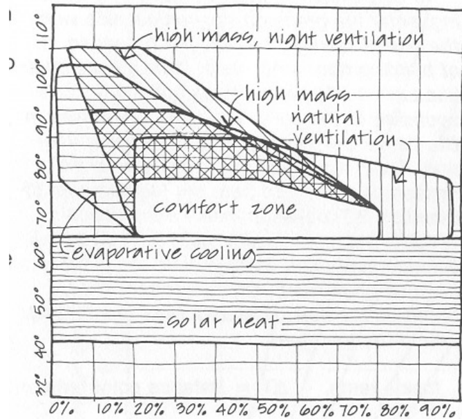
Bioclimatic Chart - Design Strategy Zones
