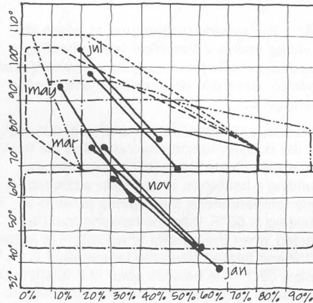
Bioclimatic Chart - Phoenix
