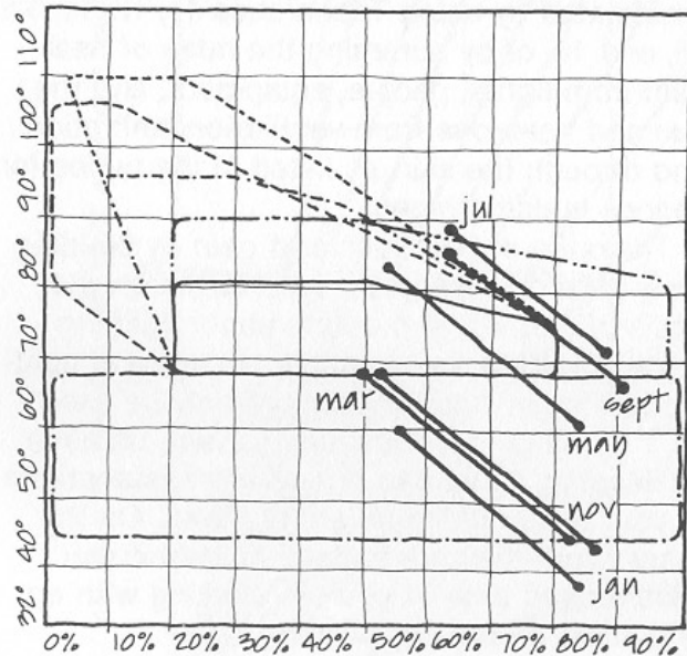
Bioclimatic Chart - Charleston
