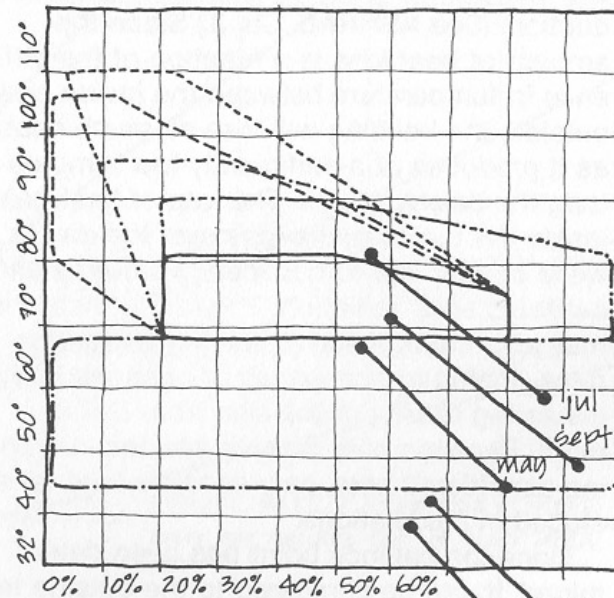
Bioclimatic Chart - Madison
