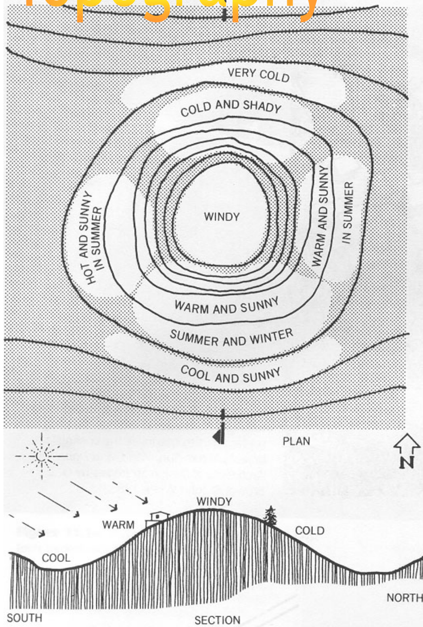
Figure 11.2c Microclimates around a hill.
